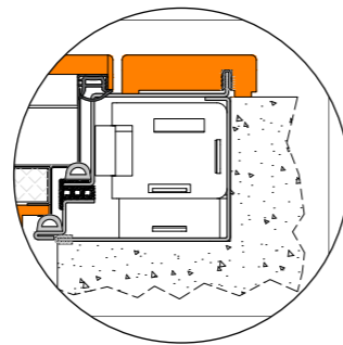
Securtherm particolare Particular Securtherm
